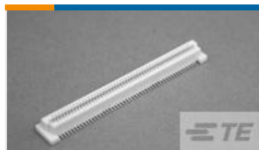
TE 产品编号7-1735480-9 0.8FH,R17H.5,180,30/Sn,TU
