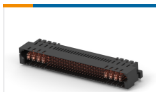
TE 产品编号2-2204910-5 MBXLE R/A HEADER 4HDP + 92S + 4HDP
