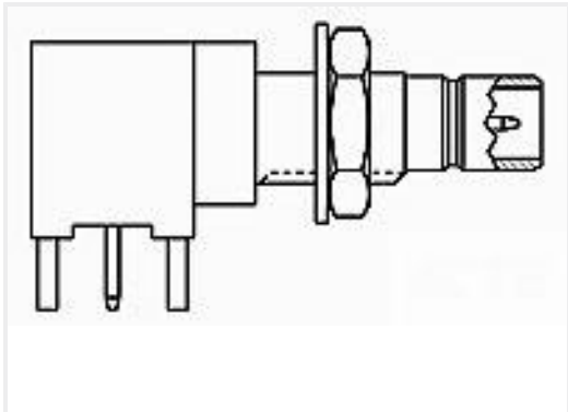
TE 产品编号415377-2 JACK, RATNG, PCB, SMB, 75 OHM
