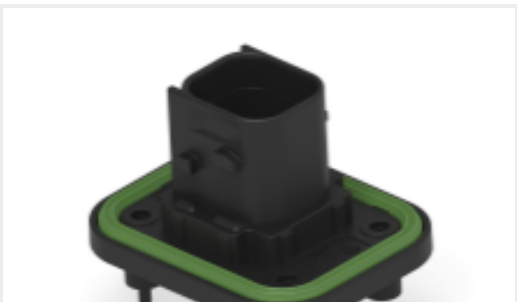
TE 产品编号1-2377473-1 4POS,TAB2.8X0.8,HDR ASSY,180DEG, COD A
