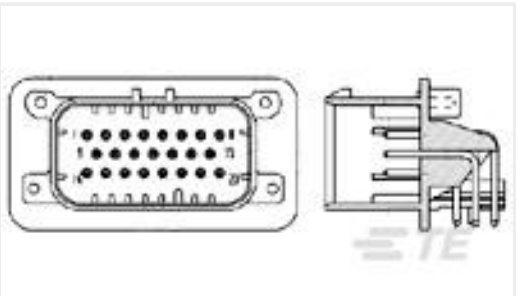
TE 产品编号776087-2 23POS,PIN DIA 1.3,HDR ASSY,90DEG, COD 2
