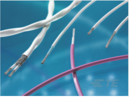
TE 产品编号CAT-55PC-S-2T-8-18 2 Core Twisted Pair Cable: Silver Coated Cable, 8-18 AWG
