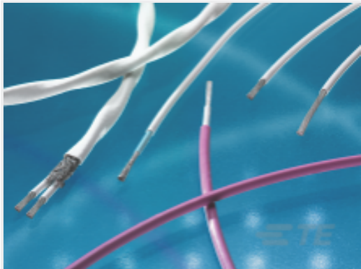
TE 产品编号CAT-55A-SC-2T-26 General Purpose 2 Core Cable: Silver Coated Cable, 26 AWG
