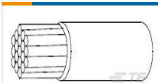
TE 产品编号216445-000 General Purpose Hookup Wire: Silver Coated Copper Wire, 22 AWG
