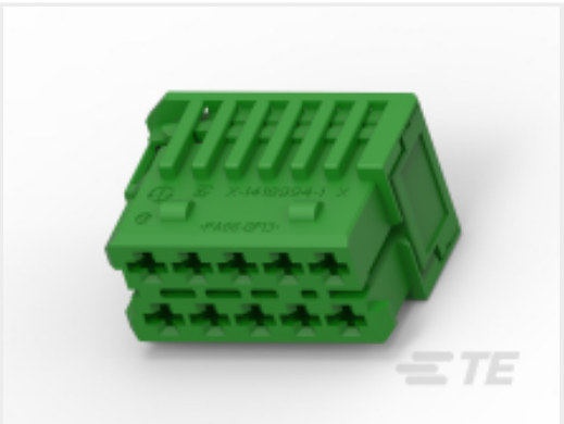
TE 产品编号3-1418994-1 AMP MCP 2.8 HSG.WITH SEC.10POS.
