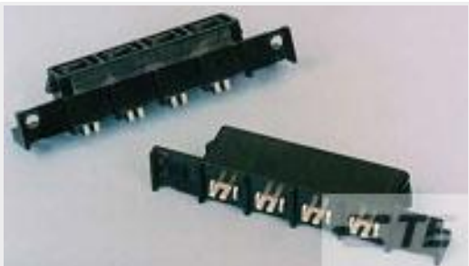
TE 产品编号556881-2 RCPT ASY,VRT,AMPINRGY WTB,2POS
