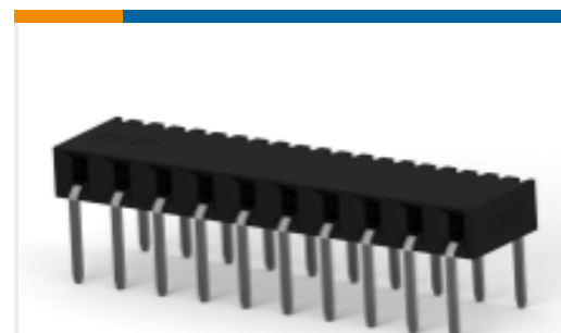
TE 产品编号1-2314938-0 10P,2MM,B-B,REC,SRHZ,2.8,0.76AU,TR
