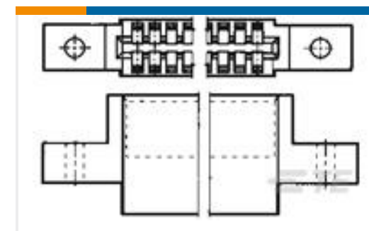
TE 产品编号1-583718-1 TW-LEAF CRP HSG 25 POS 100 C/L
