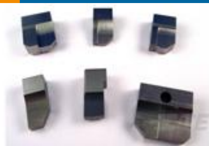
TE 产品编号1803059-6 ANVIL COMBINATION, END FEED
