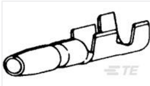
TE 产品编号61388-1 SHUR PLUG 156 20-16 AWG PTPBR
