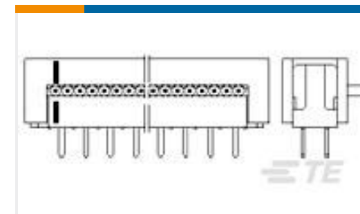
TE 产品编号1-216093-6 AMP-LATCH PRE-ASSY DIL WITHO
