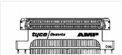
TE 产品编号 1734100-3 Champ050 series,30pos,Au over PdNi
