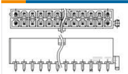
TE 产品编号3-1775099-8 ATX PWR CONN 1 BDLK 24 POS
