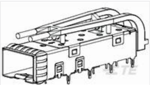
TE 产品编号 2110929-1 SFP+ 1x1 Cage Assembly, Light Pipe
