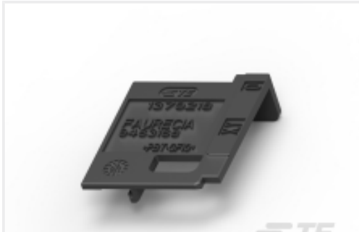
TE 产品编号1379218-1 COVER FOR 5W MPQ+MQS HSG
