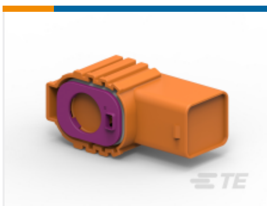
TE 产品编号2137704-2 HV1100 1POS PLUG HSG ASSY SLD 90 DEG
