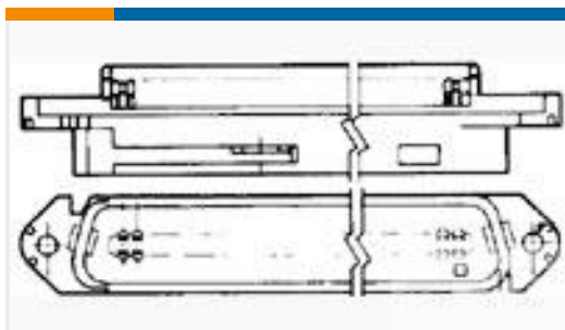
TE 产品编号229974-4 ASSY, PLUG, 50 POS, B SLOT
