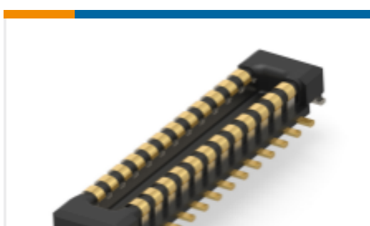
TE 产品编号2-2363962-4 0.4mm BTB CONN H0.8 PLUG ASSEMBLY, 24P
