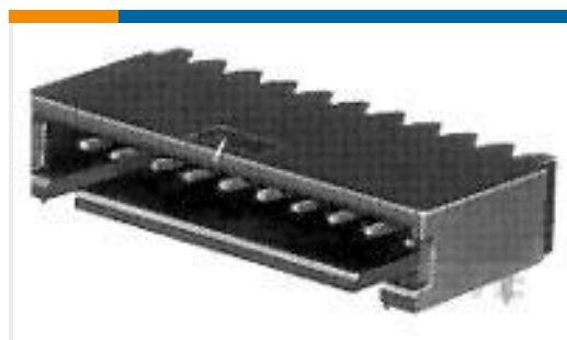
TE 产品编号5-102203-7 10 MODII HDR SRRA SHRD LF
