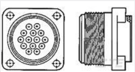
TE 产品编号213570-1 CPC RECPT 20-14 SPECIAL
