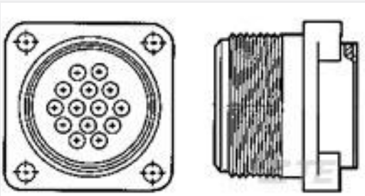
TE 产品编号213651-1 CPC RCPT 20-14 STD SEX
