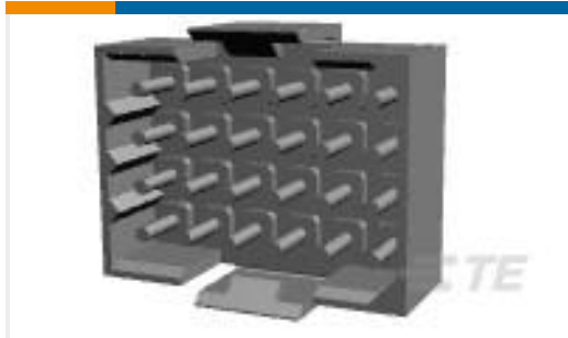
TE 产品编号1-206763-4 METRIMATE PIN HDR ASSY,24P LF
