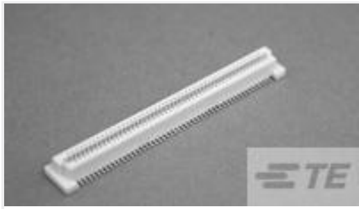
TE 产品编号1735482-3 0.8FH,R17H.5,080,08/Sn,TR,SC
