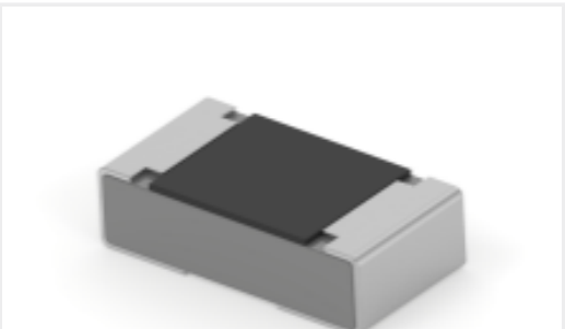
TE 产品编号2-2176479-9 RA73F 1J 100R 0.1% 5K RL
