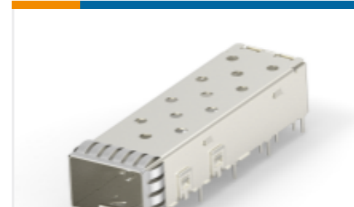
TE 产品编号 2007194-1 SFP+ 1x1 Cage Assembly, PCI, Solder Tail
