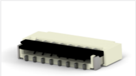
TE 产品编号1-2328724-5 15PIN 0.3MMP FPC CONNECTOR, FRONT FLIP
