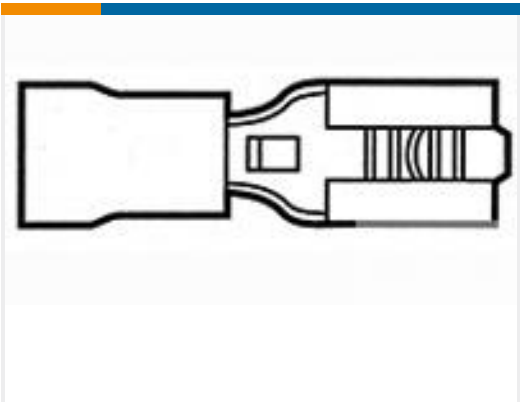
TE 产品编号696108-1 .187 PIDG FASTON REC.16-14
