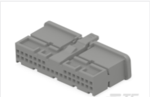
TE 产品编号2382569-2 32POS,NANOMQS,REC HSG,UNSLD, COD B,STD
