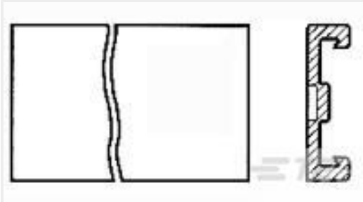
TE 产品编号640643-4 04P MTA156 COVER F/T
