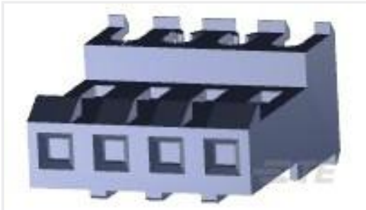
TE 产品编号3-640601-4 04P MTA156 CONN ASSY 22AWG LF
