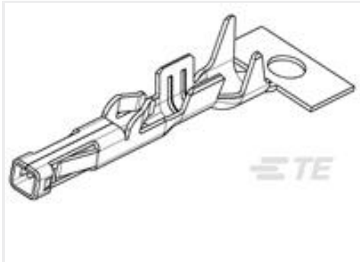
TE 产品编号1-2106123-1 CONTACT,Recept, SLC, Tin Plated, On Stri
