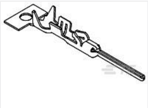
TE 产品编号2-2106124-7 Contact, Tab, Tin Plated, LP 22-16 AWG
