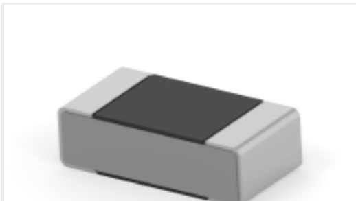
TE 产品编号3-2176236-1 CPF A 0402 20K 0.1% 25PPM 5K RL
