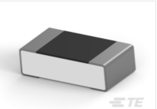
TE 产品编号2-2176365-7 RQ 0603 75R 0.1% 10PPM 1K RL
