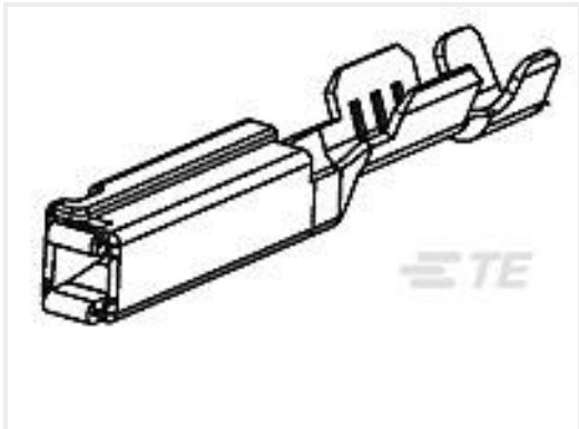
TE 产品编号1393366-2 GET-SOCKET TERMINAL, SILVER VE
