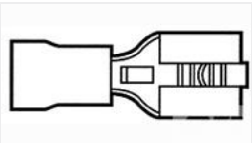
TE 产品编号55675-1 RECEPT,PIDG FASTON 22-18 250
