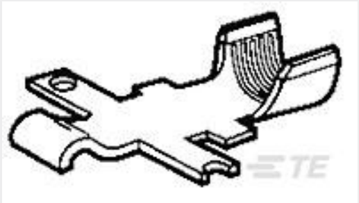
TE 产品编号53892-2 CONTACT,PWR LK,SRS1,STRIP,CRMP
