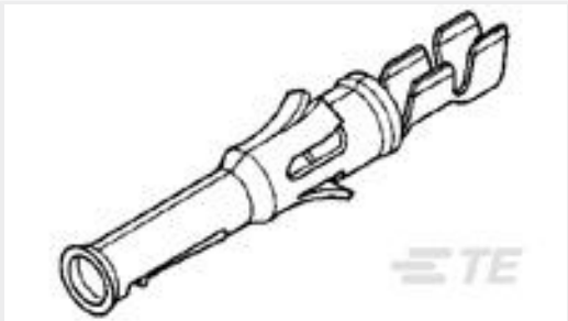
TE 产品编号66582-2 TYPE VI SKT CONT,MULTI-MATE
