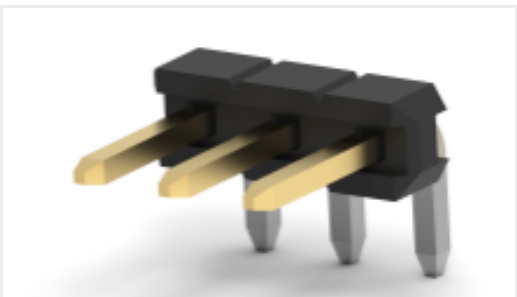
TE 产品编号2842123-3 3P,2MM,BRK HDR,SRRT,2.8,0.38AU, BOX
