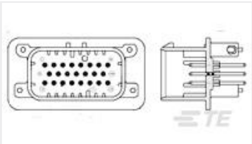
TE 产品编号776230-1 35POS,PIN DIA 1.3,HDR ASSY, 180DEG,COD 1
