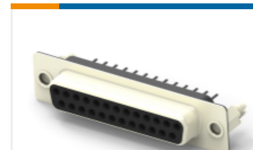
TE 产品编号2301841-1 AMPL REC HD20, VERT, 25P, B/L,4-40 INS
