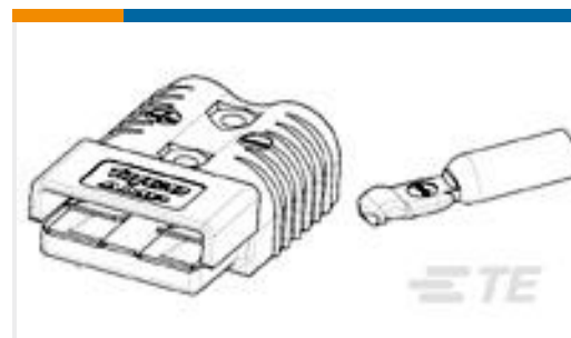
TE 产品编号1604044-4 KIT,175A, 4 AWG,GRAY
