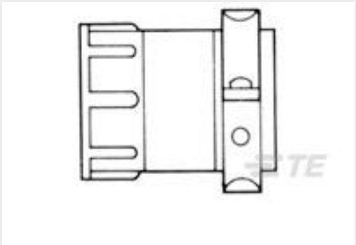
TE 产品编号206322-9 CABLE CLAMP SIZE 17
