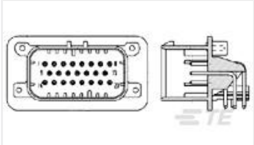
TE 产品编号1-770669-5 23POS,PIN DIA 1.3,HDR ASSY,90DEG, COD 5
