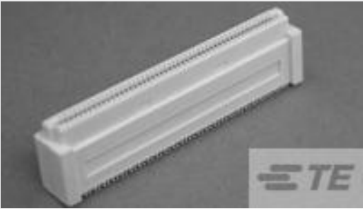
TE 产品编号1-2332208-3 RECEPT ASSY, RA, 56 POS, SLIVER 2.0
