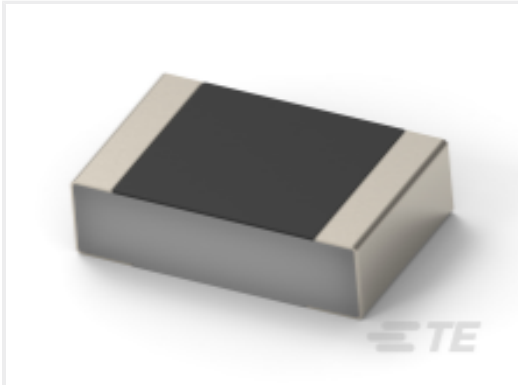
TE 产品编号5-2176074-8 CPF 0201 22K6 0.5% 50PPM 1K RL
