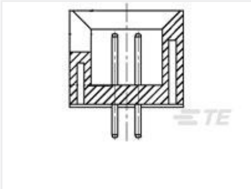
TE 产品编号1759500-8 BLIND MATE BOX HEADER 8P
