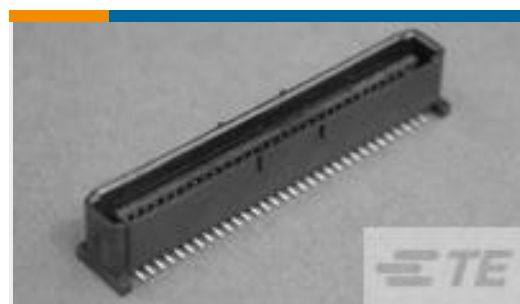
TE 产品编号5120525-1 1FHP,64,30A/S,S,N,S08
