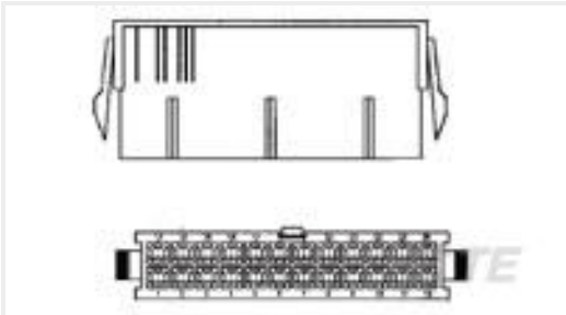
TE 产品编号1-794953-6 16P PM PLUG VAL-U-LOK V2
